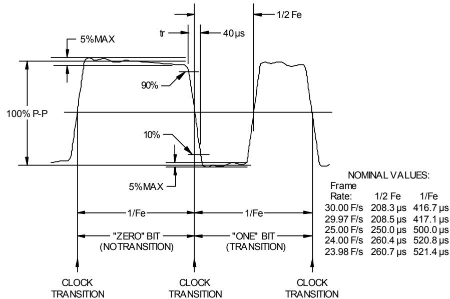
Figure 1 – Linear time code source output waveform
