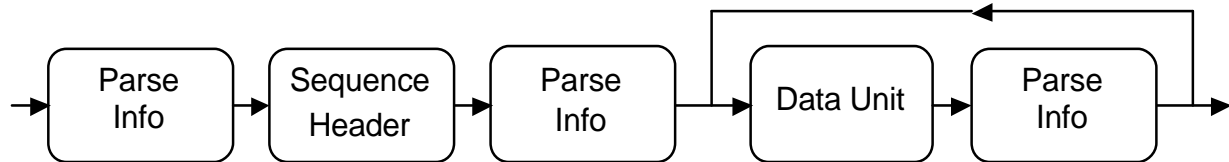
Figure 10.2 – Overview of VC-2 sequence structure
