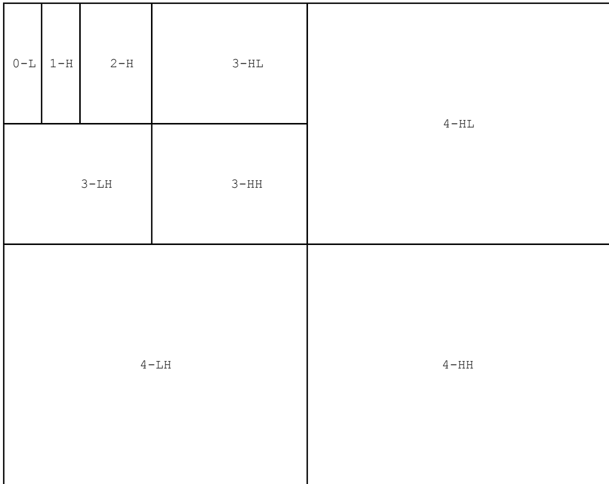
Figure 8.4 – Identification of the subbands of a 2-level 2D plus 2-level 1D wavelet transform
