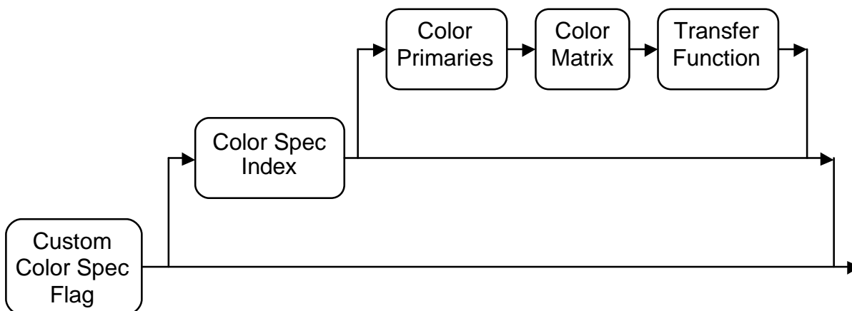
Figure 11.11 – Color specification syntax
