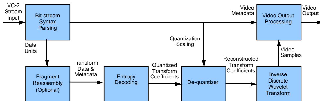
Figure 9.1 – Functional VC-2 decoder block diagram
