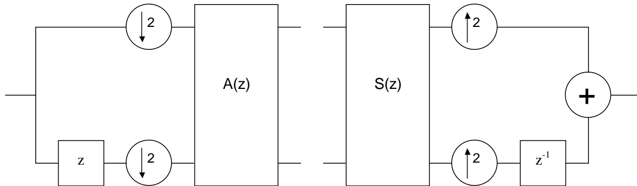
Figure F.6 – Polyphase representation of wavelet filter banks
