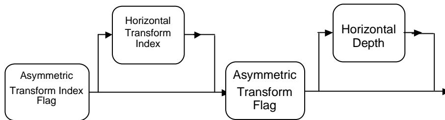
Figure 12.4 – Extended Transform Parameters
