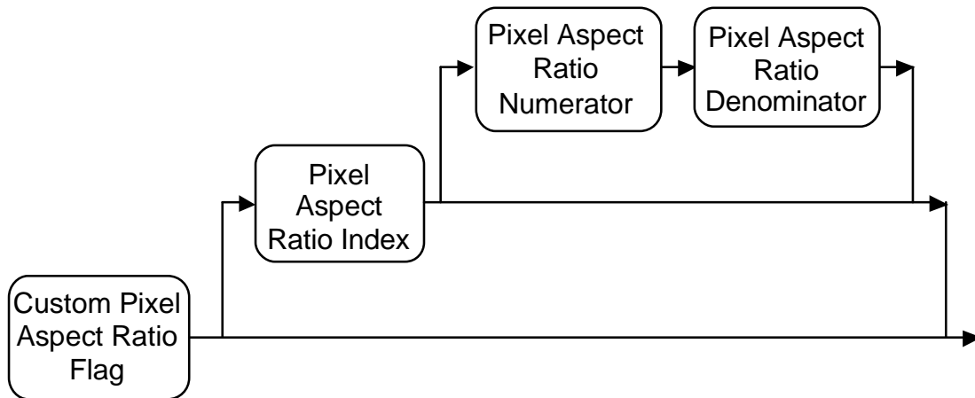
Figure 11.8 – Pixel Aspect Ratio
