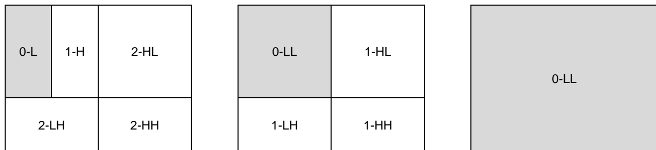
Figure 9.4 – Wavelet Decoding Steps (Combined 1D and 2D)
