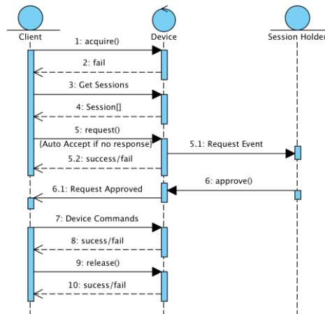
Figure 5 – Requesting a Session
