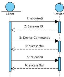
Figure 3 – Acquiring a Session
