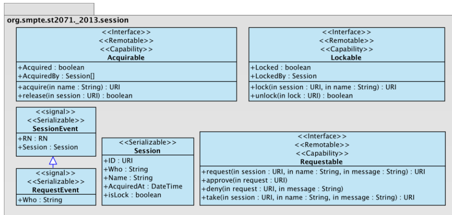
Figure 12 – Session and Lock Management
