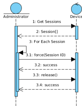
Figure 7 – Administration of Sessions and Locks
