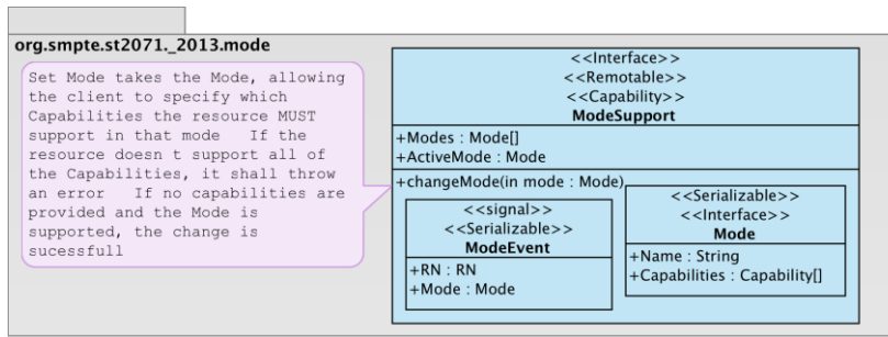
Figure 13 – Modes Framework UML Diagram
