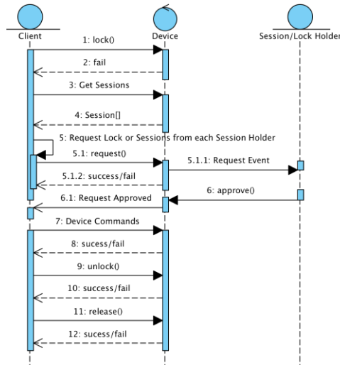
Figure 6 – Requesting an Exclusive Lock
