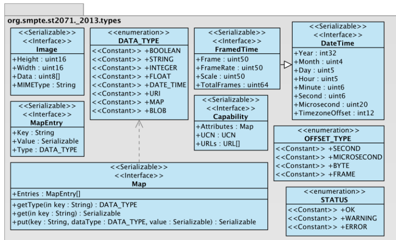
Figure 15 – Data Types UML Diagram
