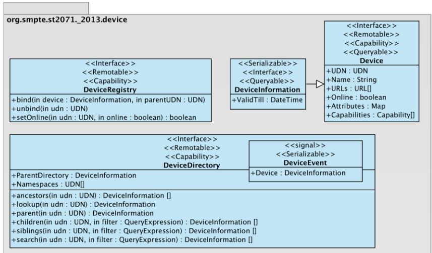
Figure 11 – Device Framework UML Diagram
