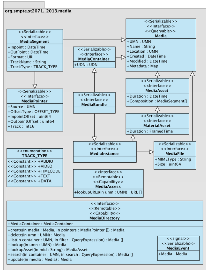
Figure 14 – Media Framework UML Diagram
