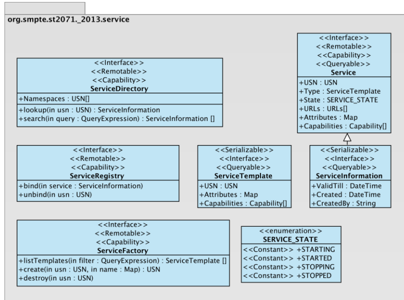
Figure 10 – Service Framework UML Diagram
