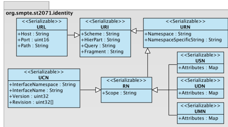
Figure 8 – Identity UML Diagram
