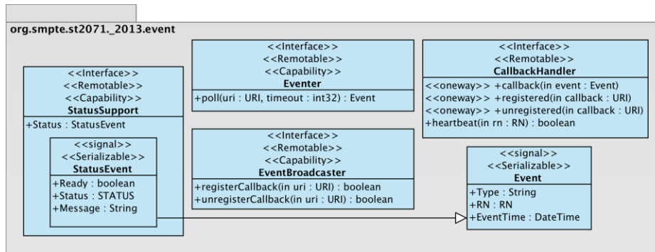
Figure 9 – Status and Events UML Diagram
