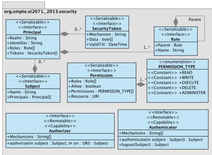
Figure 17 – Security Framework UML Diagram
