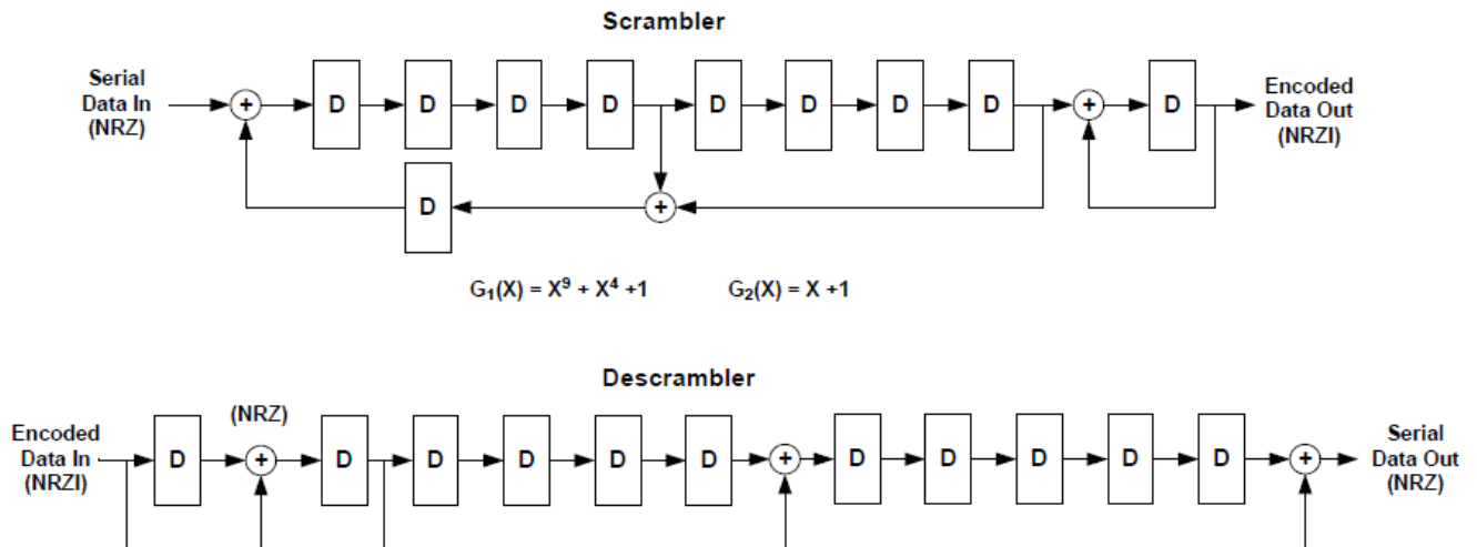
Figure B.2 – Possible Generator polynomial – Method 2
