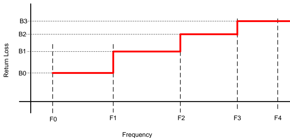
Figure 5 – Return loss
