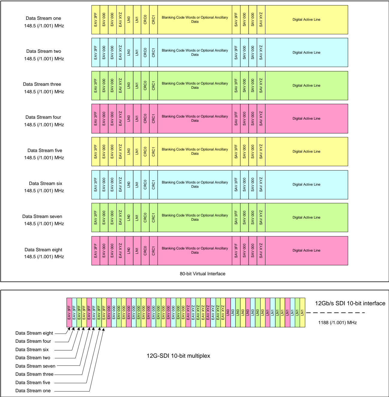
Figure 1 – 12G-SDI 10-bit Multiplex – Type 1
