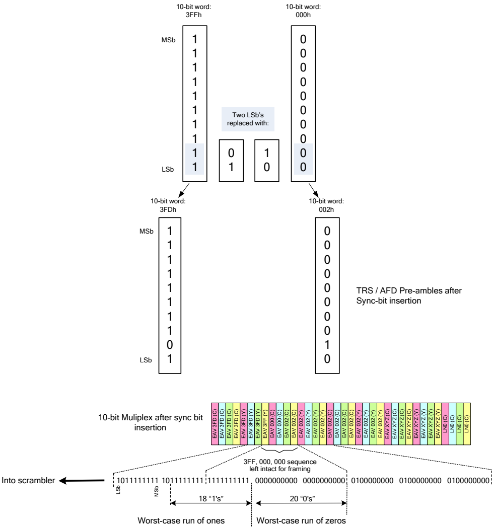
Figure 3 – Sync-bit Insertion process
