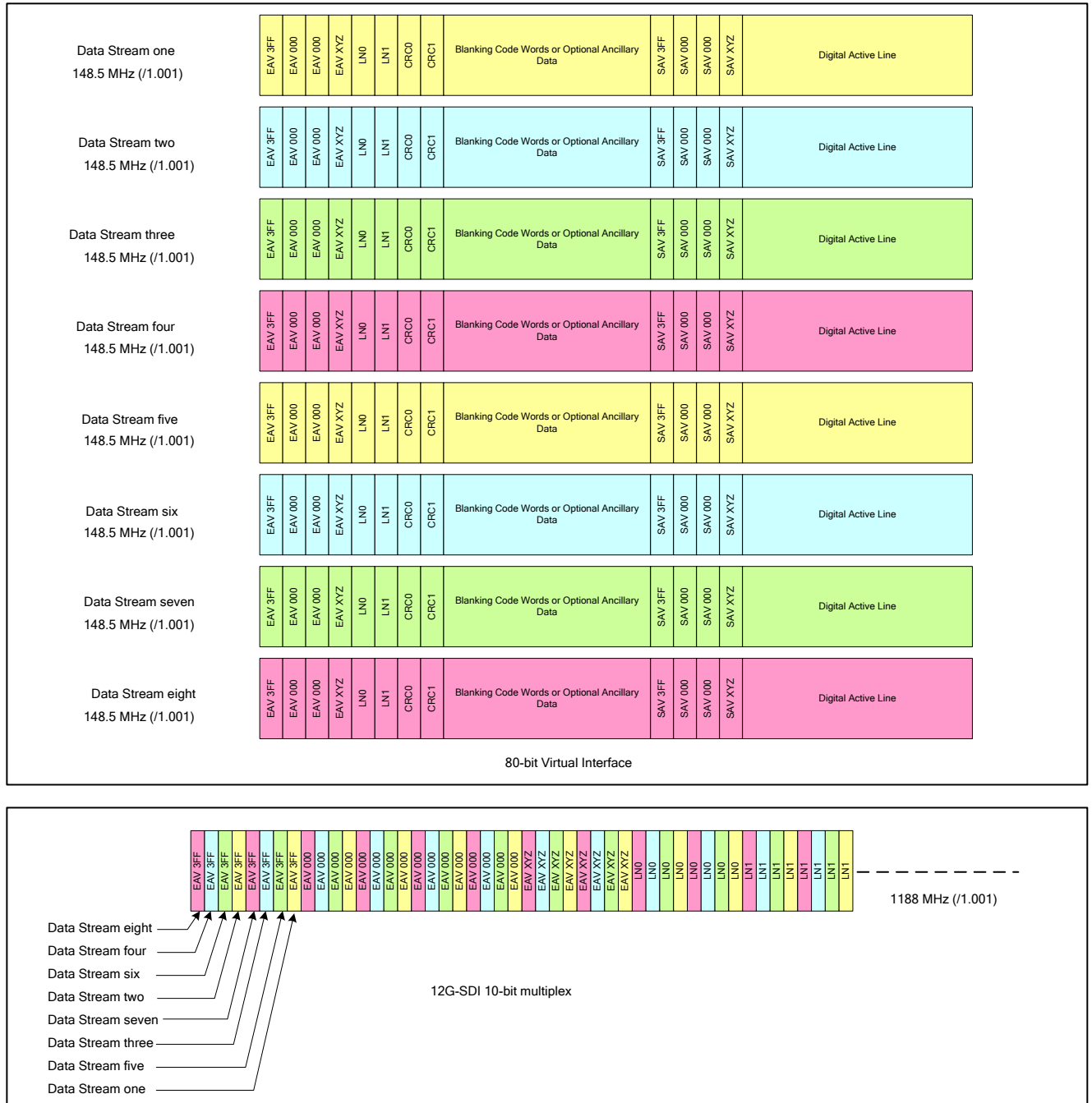
Figure 9 – 12G-SDI 10-bit Multiplex Type 1 for Mode 1 and Mode 2
