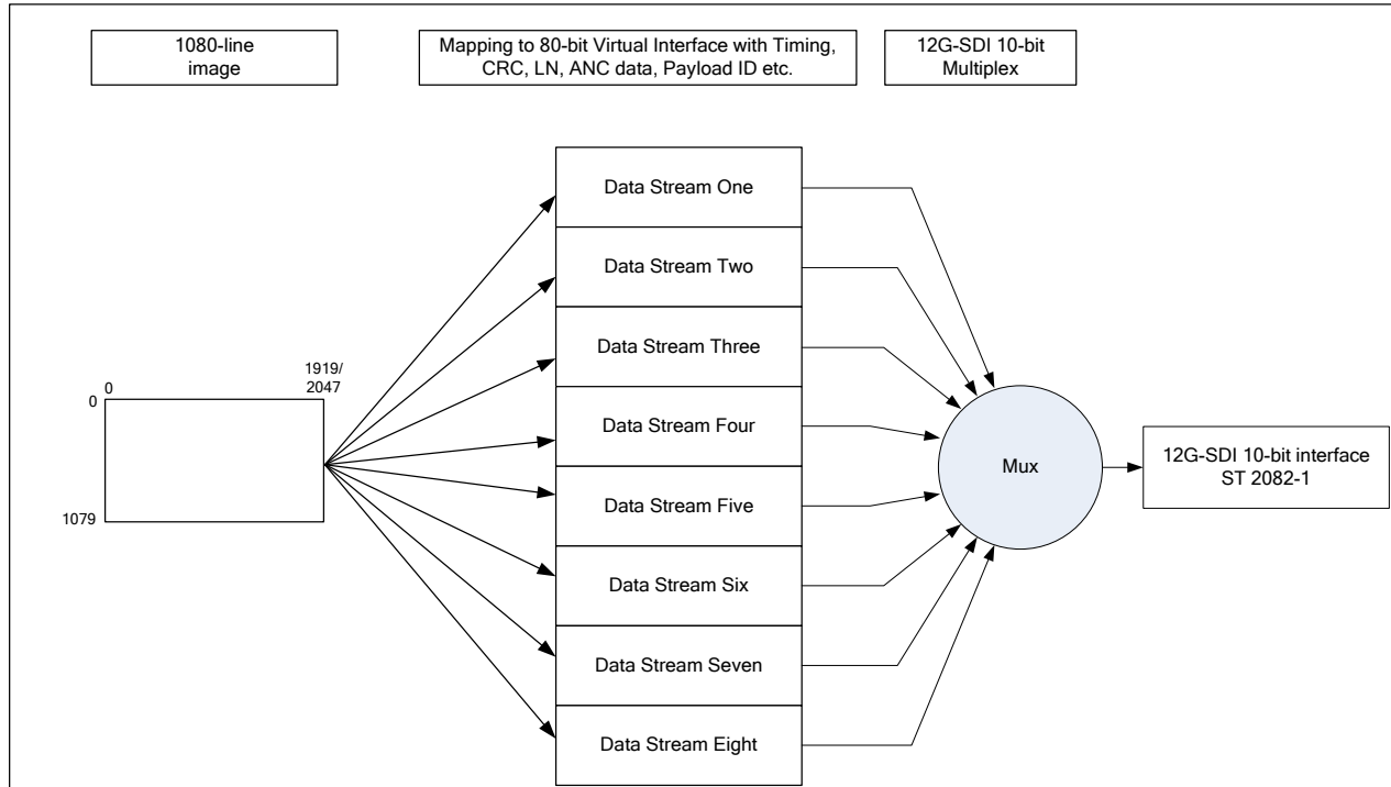
Figure 6 – Carriage of 1080-line HFR image on a 12G-SDI interface – overall process
