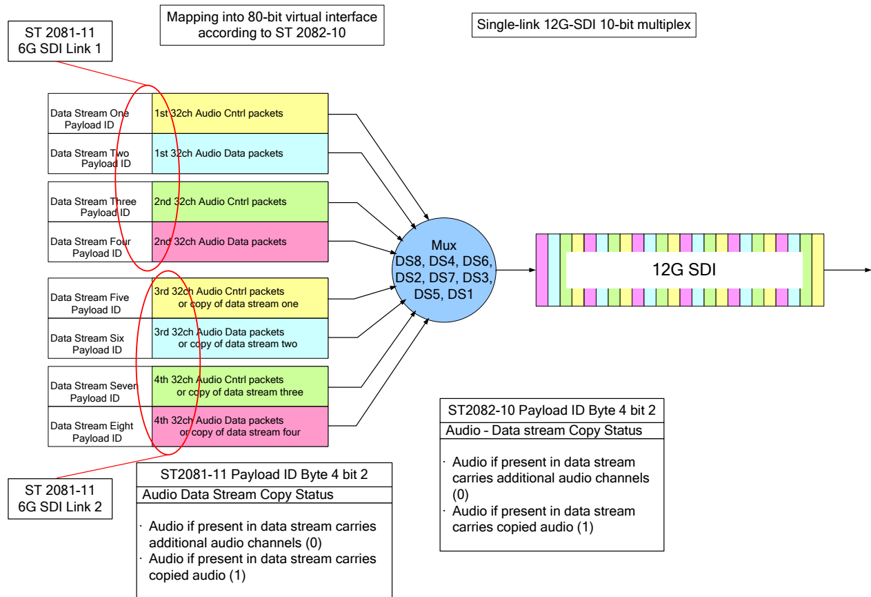
Figure 5 – Inherited audio copy as a result of combining a dual-link 6G-SDI signal
