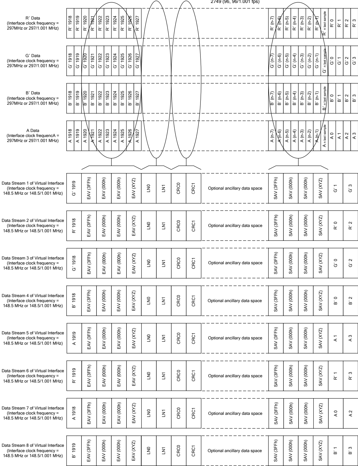
Figure 8 – Mapping Structure II 1920 x 1080 4:4:4 R'G'B'(A)/10-Bit Signals at 96/1.001, 96, 100, 120/1.001 and 120 Progressive Frames/Sec
