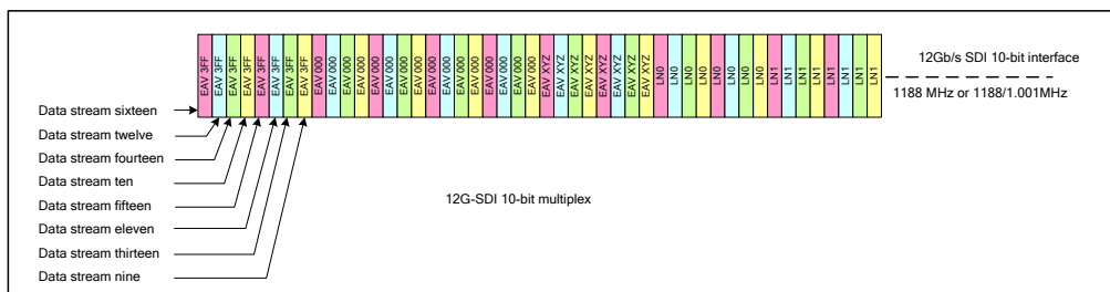
Figure 9 – Dual-link 12G-SDI 2 x 10-bit Multiplex – Type 1
