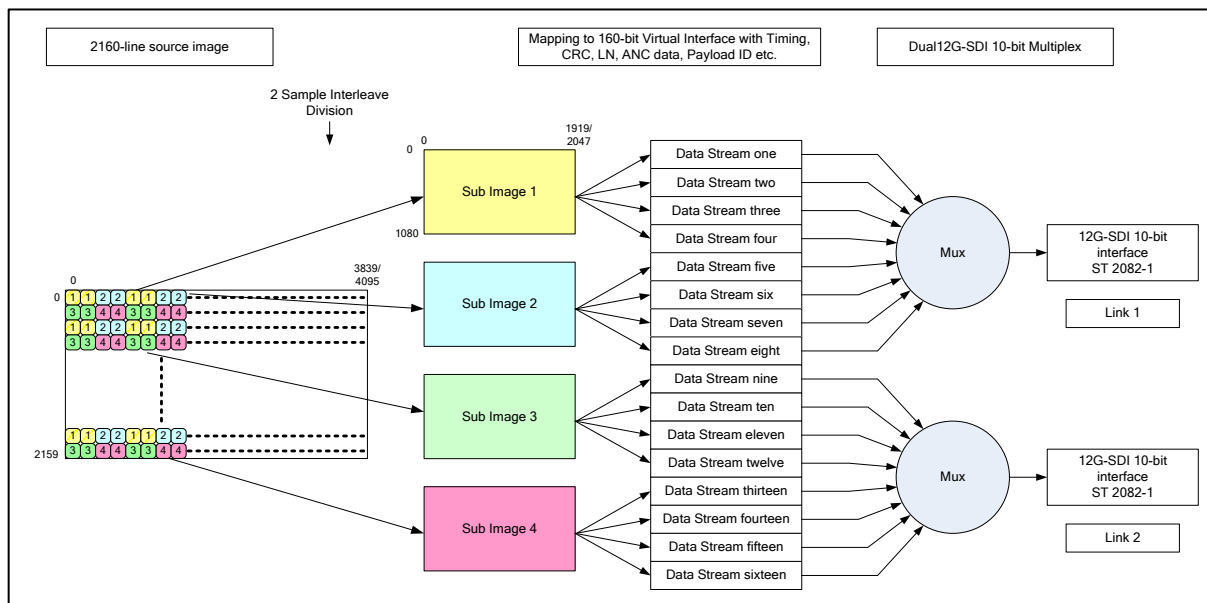
Figure 5 – Carriage of 2160-line image formats in a dual-link 12G-SDI interface
