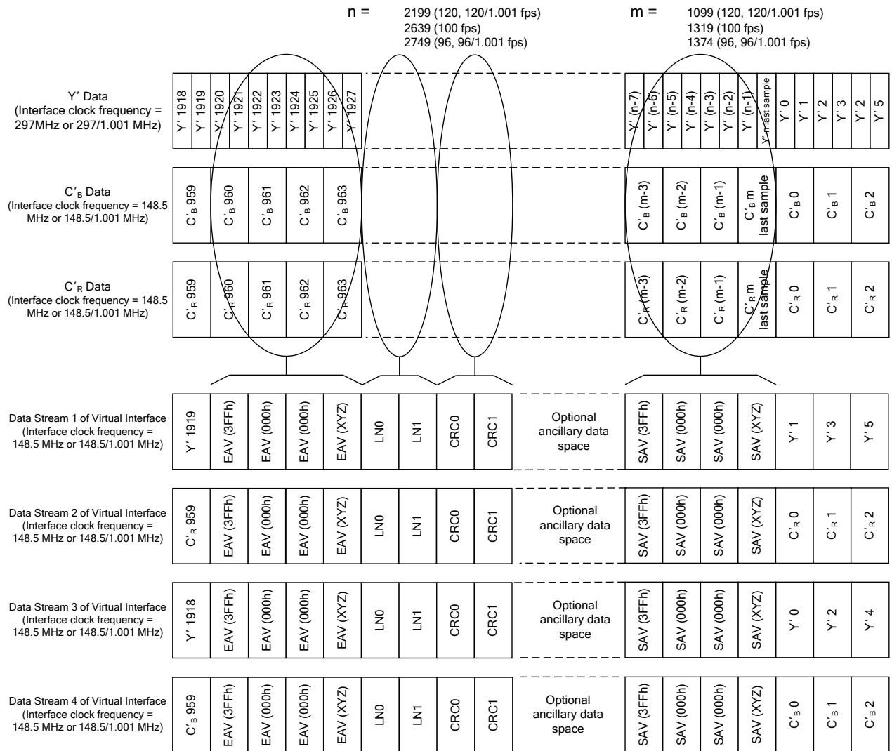
Figure 8 – Mapping Structure 4:2:2 (Y'C'B'C'R)/10-Bit Signals at 96, 96/1.001, 100, 120 and 120/1.001 Progressive Frames/Sec – Sub image 1
