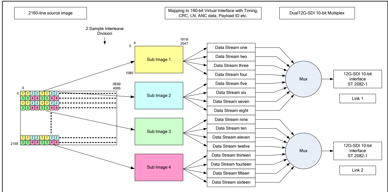
Figure 6 – Carriage of 2160-line image formats in a dual-link 12G-SDI interface
