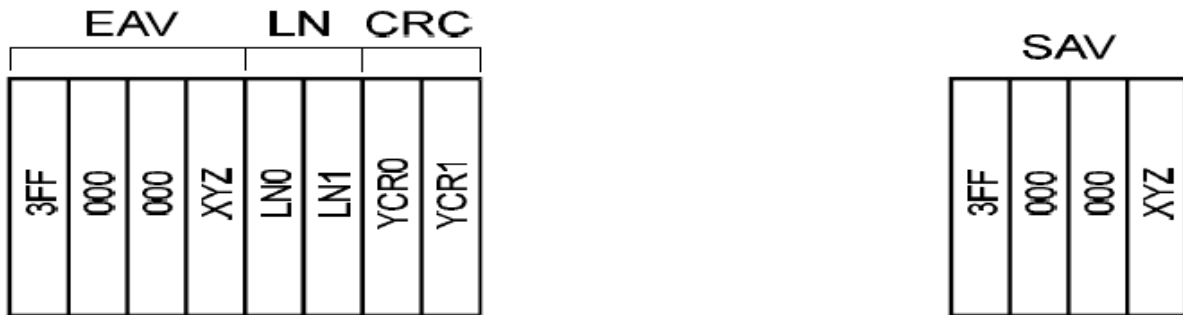
Figure 2 – Timing reference format (Luma channel shown)
