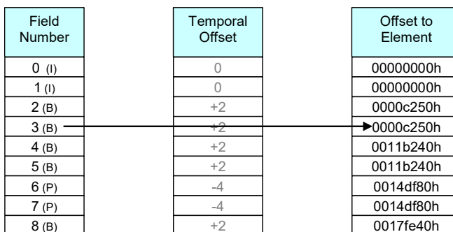
Figure 27 – Conversion from Field Number to Offset ignoring Temporal Offset
