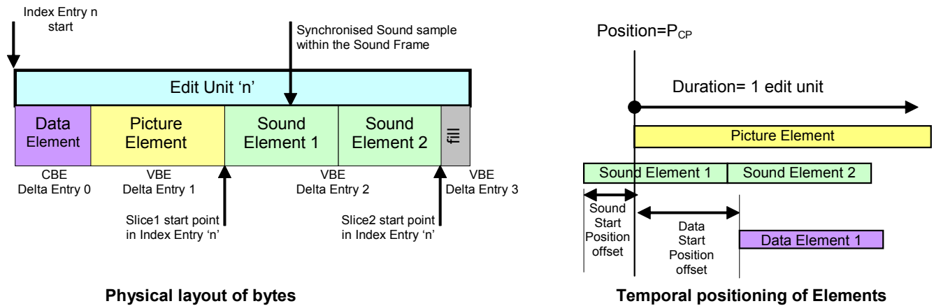
Figure A.3 – Content Package for Index Table VBE Example
