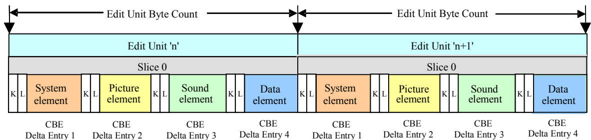
Figure A.1 – Index Table Relationships for Frame Wrapped CBE MPEG Essence
