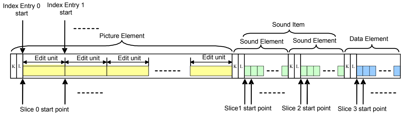
Figure A.2 – Index Table Relationships for Clip Wrapped CBE MPEG Essence
