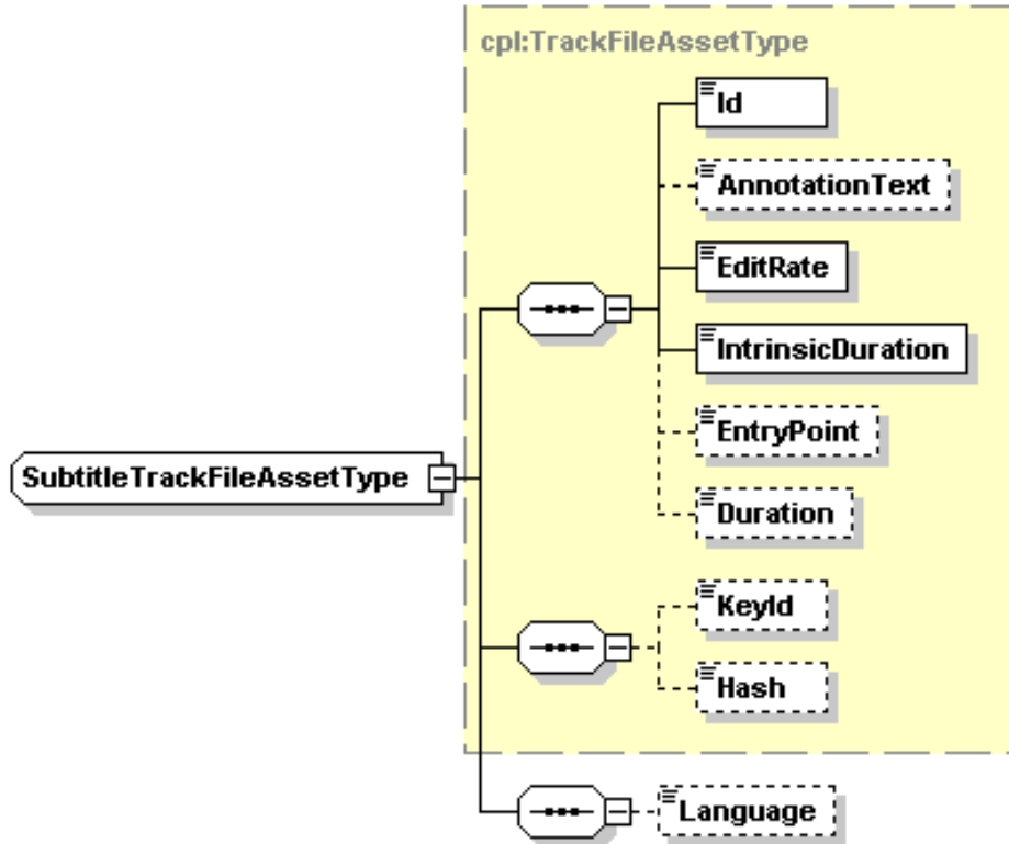
Figure 15 – Subtitle Track File Asset structure (Dotted lines denote an optional element)
