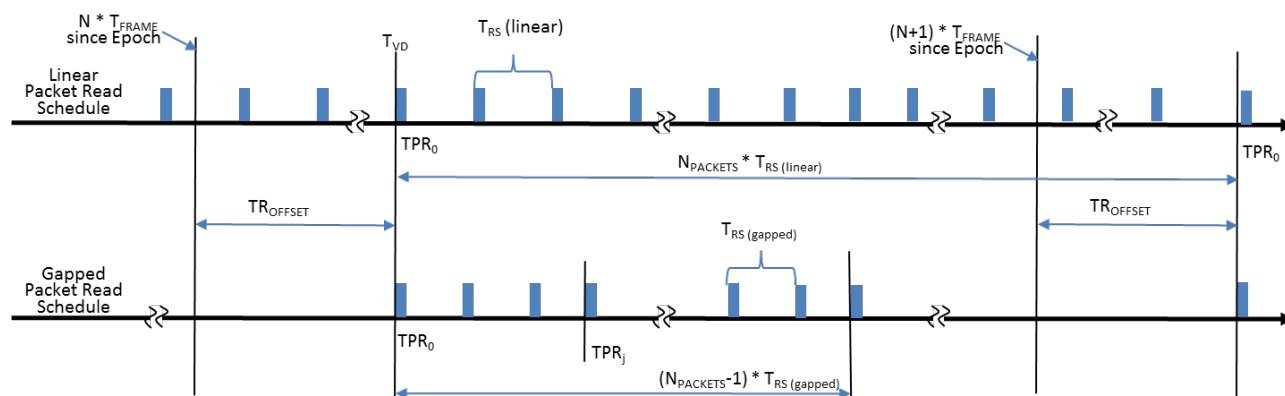
Figure 3 — Relationship between the Linear and Gapped PRS
