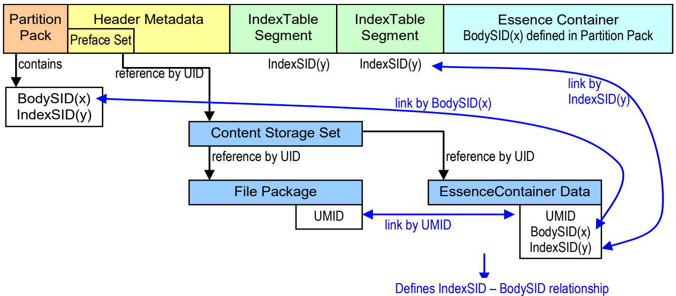
Figure 17 – Relationship between BodySID and IndexSID
