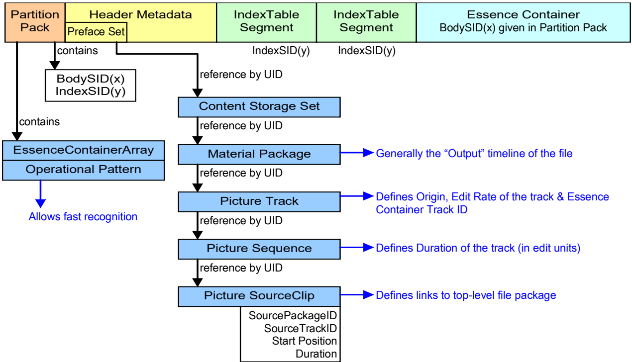
Figure 15 – Relationship between Material Package references
